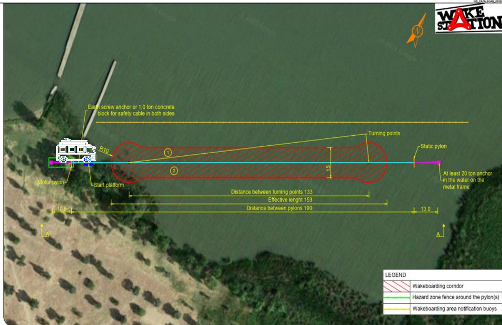
WAKESTATION CARI F PARK SITE PLAN (M 1:1000)
