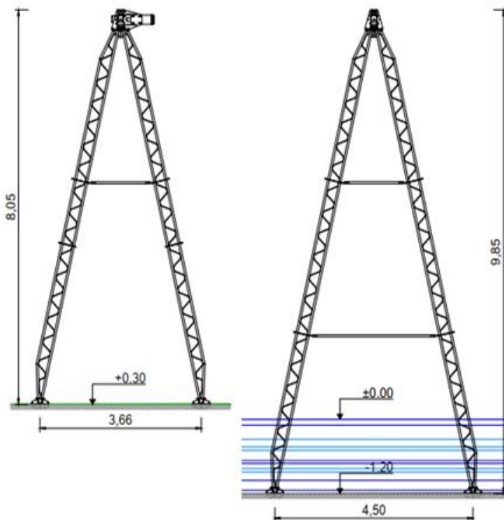
FRONT VIEW OF PYLON WS805 AND WS985 (M 1:100)
